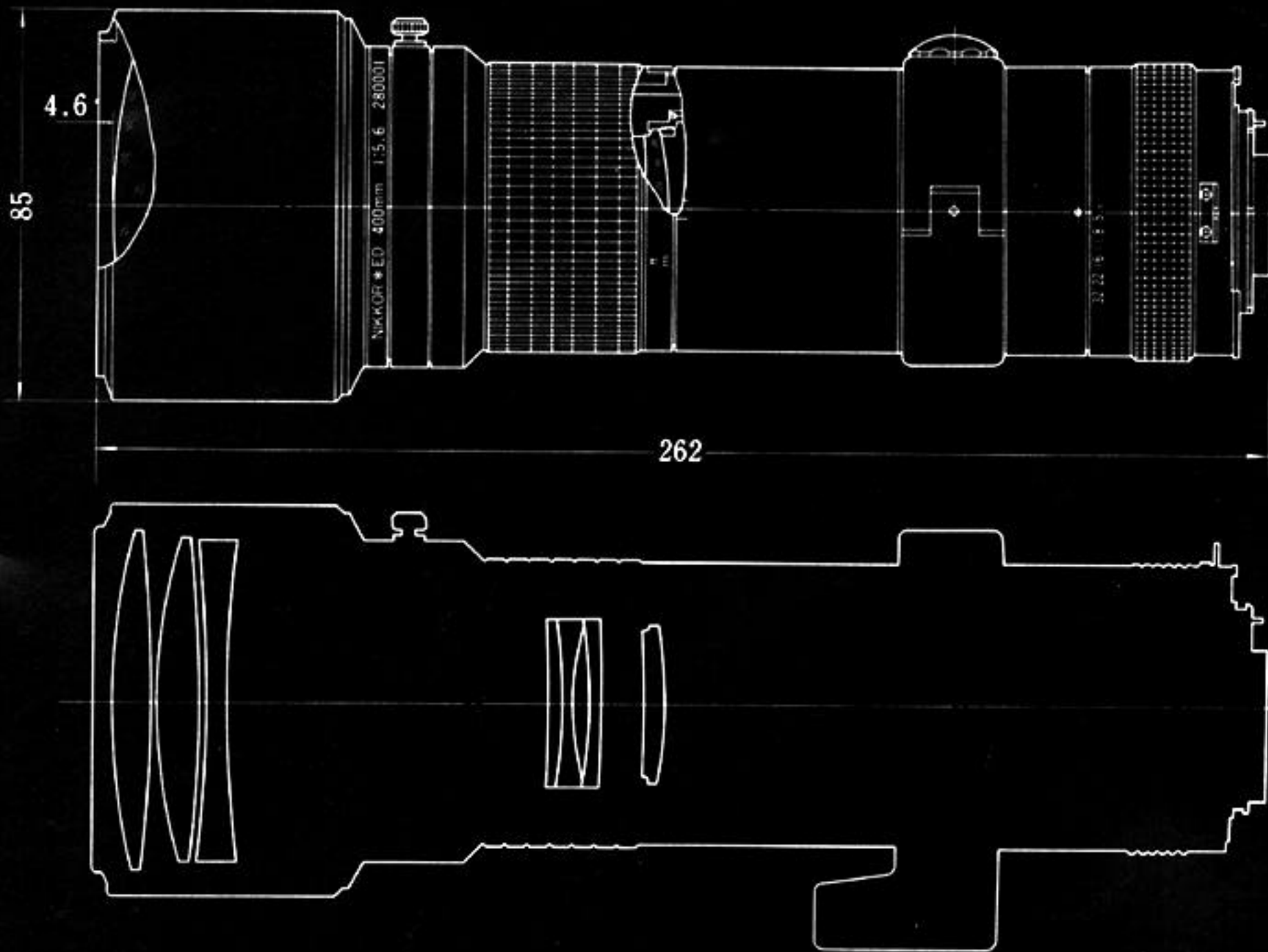
Nikkor 400mm f/5.6 IF-ED
