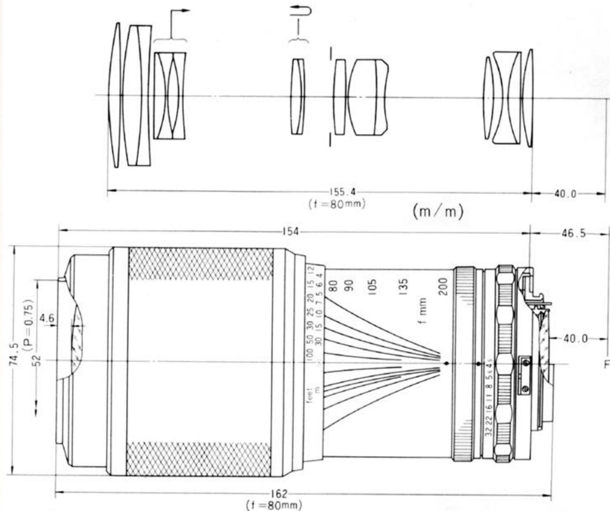
Non-Ai Zoom Nikkor Auto 1:4.5 f=80mm~f=200mm lense
